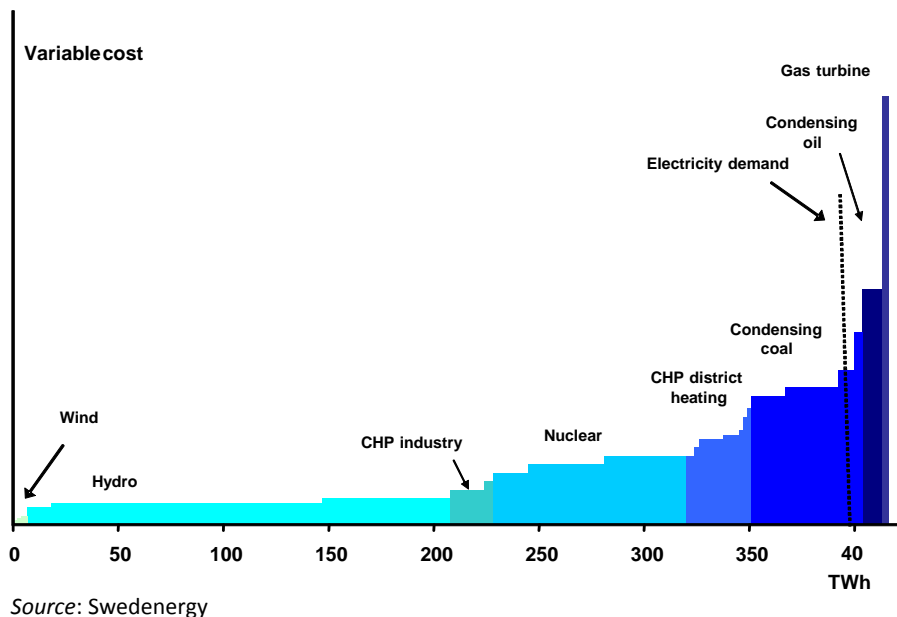
Figure 1: Principal Merit Order Curve in the Nordic Electricity Market
